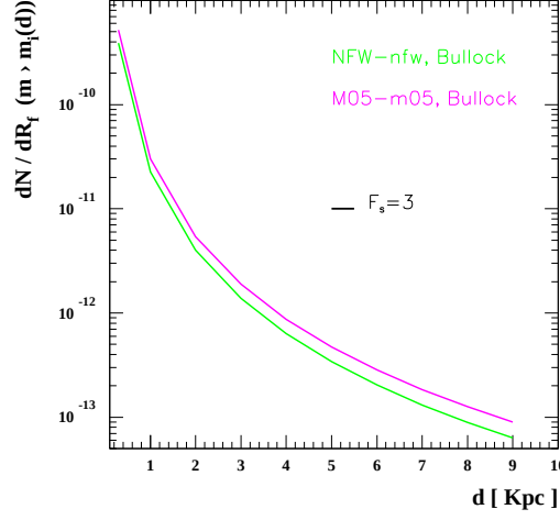
Figure 5.3: Probability of finding a clump of mass m_i at the final distance d according to subhalo distribution model discussed in Chapter 2. Figure by Bisesi & Ullio, 2007 [42].
