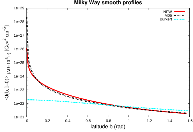
Figure 4.3: Behavior of the \langle J(l, b) \rangle_{smooth} term with the Galactic latitude b , for different halo profiles and the instrumental PSF of the MAGIC experiment ( \Delta\Omega = 10^{-5} sr).
