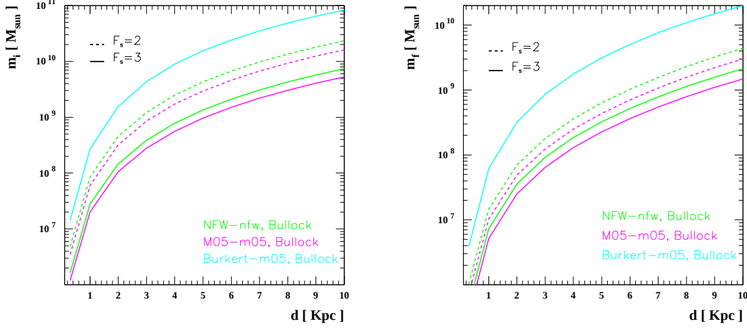
Figure 5.2: Initial ( left panel ) and final ( right panel ) subhalo mass versus the heliocentric distance for the unidentified EGRET source 3EG_J1835 + 5918 for different choices of the progenitor profile and concentration model. Figure by Bisesi & Ullio, 2007 [42].
