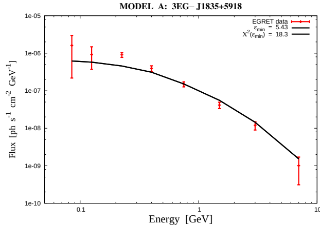
Figure 5.1: EGRET measured differential fluxes (red) for the unidentified gamma-ray source 3EG-J1835+5918. Data taken from http://heasarc.gsfc.nasa.gov/db-perl/W3Browse/w3browse.pl . Fit with the SUSY model as in Table (5.3).
