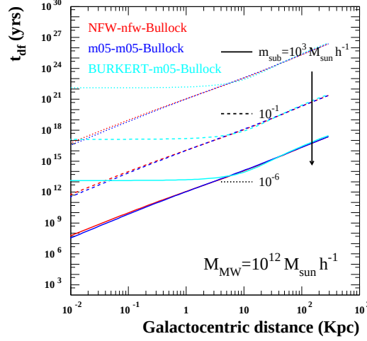
Figure 2.6: Behavior of the dynamical friction time with the distance from the center of the Milky Way, for different subhalo masses and models considered in Fig. 2.4 and 2.5. Figure by Bisesi & Ullio, 2006 [42].
