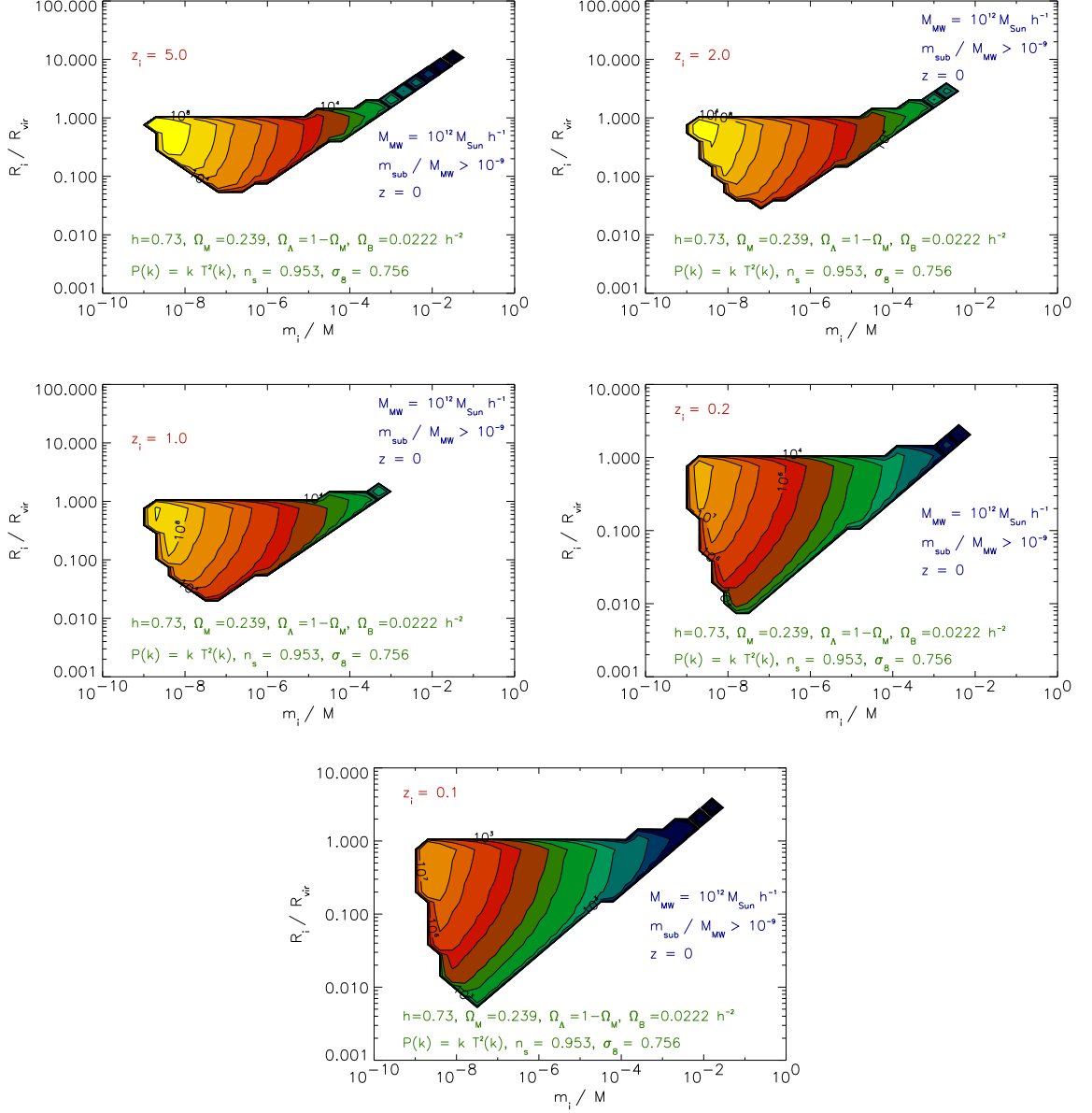
Figure 2.7: The MW subhalo population final configuration region, in the (m_i, R_i) plane, for fixed values of z_i ; z_i = 5 ( upper left ), z_i = 2 ( upper right ), z_i = 1 ( middle left ), z_i = 0.2 ( middle right ), and z_i = 0.1 ( lower ). We plot contours of the mass and spatial distribution function of subhalos, weighted on their formation epoch distribution, (dp/dz_i) d^2 N_{M,z,z_i}/dR_i dm_i , in a logarithmic space. Yellowish contours mean larger values, thus corresponding regions contribute to the distribution function more. The adopted cosmological parameters, as well as the slope of the power spectrum, are shown on the bottom of each panel (Erica Bisesi, 2006).
