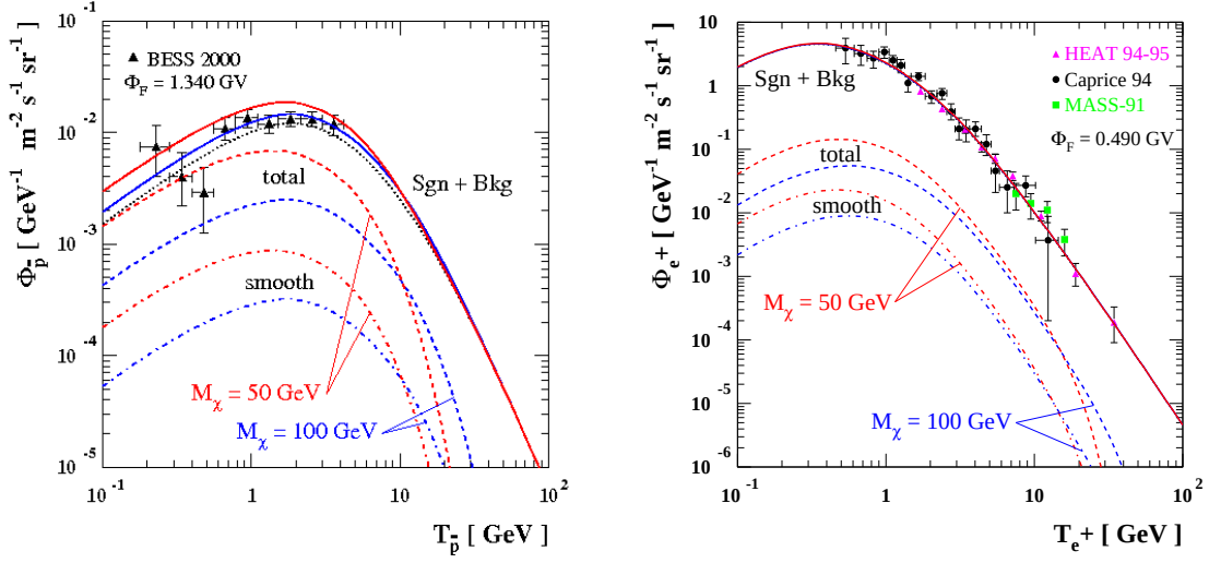
Figure 4.7: The antiproton ( left panel ) and positron ( right panel ) fluxes for two sample WIMP models with given annihilation rate (simplified scaling with the inverse of the relic density value), dominant annihilation final state into b\bar{b} and mass M_\chi = 50 GeV or 100 GeV. The configuration for the substructure distribution is the one obtained assuming a NFW universal shape profile and concentration parameter in substructures being twice the concentration in halos of equal mass (parameter F_s = 2 ) as extrapolated with the Bullock et al. prescription. In each case, a dashed-dotted line is used for the contribution from the smooth halo component only, a dashed line for the total flux from WIMP annihilations, while a solid line for the sum of the signal and background contributions; all fluxes displayed are solar modulated and data taken at the corresponding phase of the solar cycle are plotted. Figure by Bisesi & Ullio, 2007 [42].
