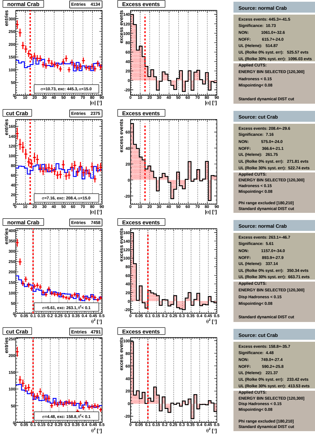
Figure 9.8: Alpha and Theta-squared plots for the normal Crab . (Courtesy of the MAGIC Collab.).
