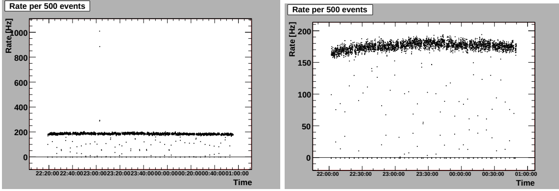
Figure 8.3: Plots of rate versus time for the ON and OFF data. The ON run 46693 has been moved out by hand.
