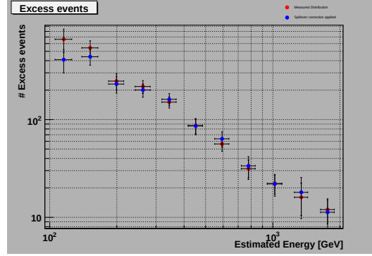
Figure 8.10: Distribution of the excess events calculated from the \alpha -plots.
