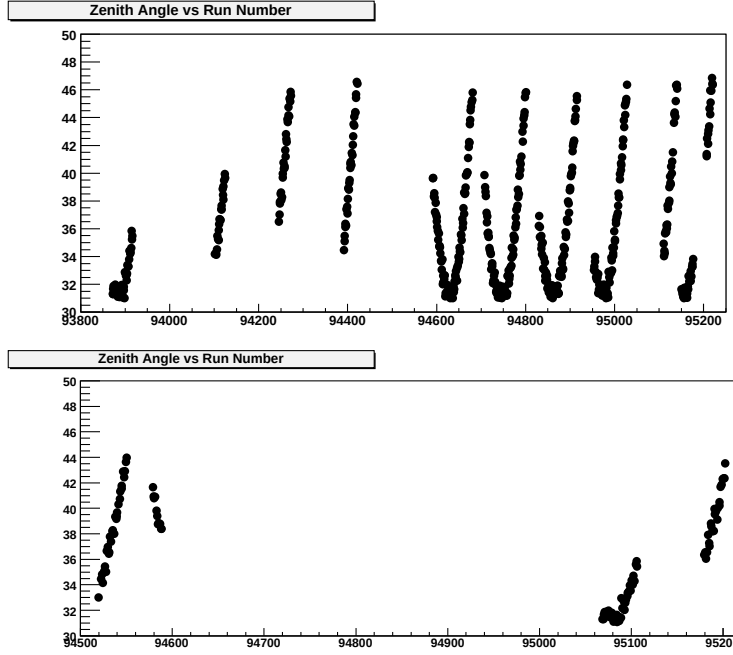
Figure 9.2: The zenith angle of the data vs run number for ON and OFF data. (Courtesy of the MAGIC Collab.).
