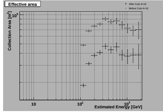
Figure 8.11: Effective area.
