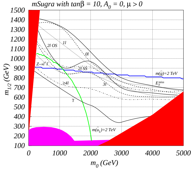
Figure 3.3: An example of the reach of the Large Hadron Collider (LHC) to new TeV-scale physics. The red regions are excluded by theoretical constraints, while the magenta region is excluded experimentally. 100 \text{ fb}^{-1} of integrated luminosity is assumed. Figure by [39].
