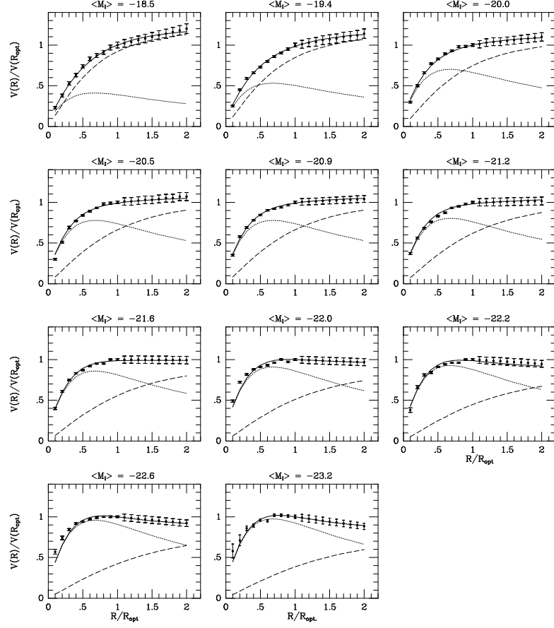
Figure 2.2: Synthetic rotation curves (circles) and the Universal Rotation Curve (solid line). The dark/luminous contributions are indicated with a dashed/dotted line. Figure by [172].
