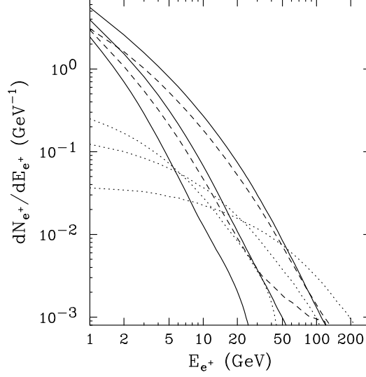
Figure 4.4: The positron spectrum from neutralino annihilations for the most important annihilation modes. Solid lines represent the positron spectrum, per annihilation, for \chi^0\chi^0 \rightarrow b\bar{b} , for LSPs with masses of 50, 150 and 600 GeV. The dotted lines are the same, but from the process \chi^0\chi^0 \rightarrow \tau^+\tau^- . Dashed lines represent positrons from the process \chi\chi \rightarrow W^+W^- for LSPs with masses of 150 and 600 GeV. The spectrum from \chi\chi \rightarrow ZZ is very similar. Figure by [39].
