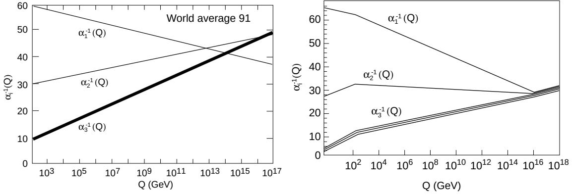
Figure 3.1: The measurements of the gauge coupling strengths at LEP do not ( left panel ) evolve to a unified value if there is no SUSY, but do ( right panel ) if SUSY is included. Figure and text from [39].
