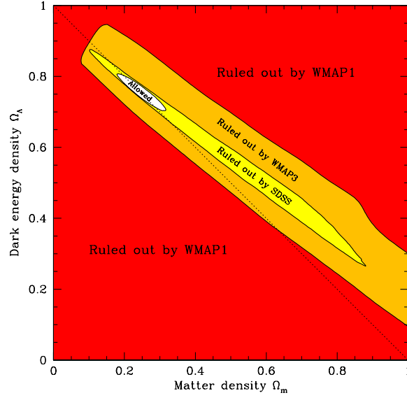
Figure 1.2: Constraints on the geometry of the Universe in the (\Omega_M, \Omega_\Lambda) plane from the CMB anisotropies as measured by the WMAP satellite.
