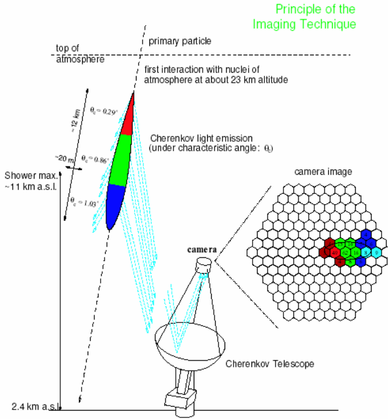
Figure 6.7: The Čerenkov technique, through the formation of the image of an electromagnetic air shower in an IACT pixelized camera for a typical 1 TeV gamma-ray induced shower.
