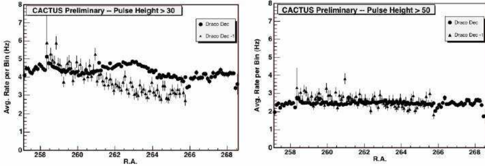
Figure 10.7: Average rate observed by the CACTUS Telescope in the direction of Draco; pulse height cuts of 30 ( left panel ) and 50 ( right panel ) have been applied. A pulse height of 50 is of the order of 100 GeV. Figure by [28].
