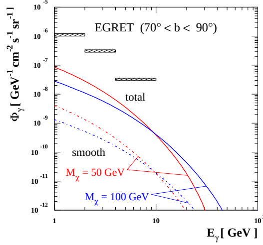
Figure 4.6: The high latitude gamma-ray flux for two sample WIMP models with given annihilation rate (simplified scaling with the inverse of the relic density value), dominant annihilation final state into b\bar{b} and mass M_\chi = 50 GeV or 100 GeV; in this plot as well the configuration for the substructure distribution is the one obtained assuming a NFW universal shape profile and concentration parameter in substructures being twice the concentration in halos of equal mass (parameter F_s = 2 ), as extrapolated with the Bullock et al. prescription. A dashed-dotted line is used for the contribution from the smooth halo component only, while a solid line for the total flux from WIMP annihilations; data for the high latitude flux collected by the EGRET experiment are shown for comparison. Figure by Bisesi & Ullio, 2007 [42].
