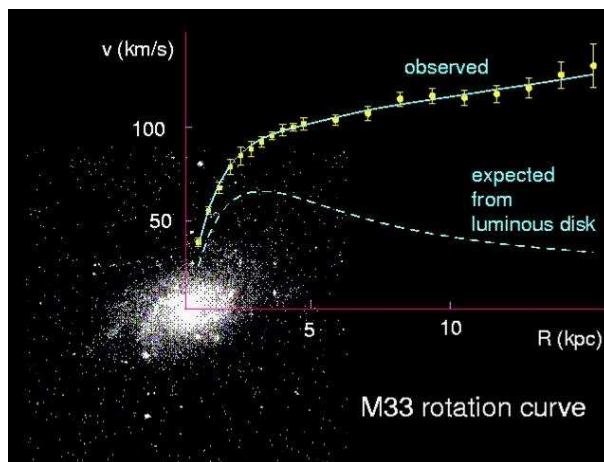
Figure 1.1: An optical image of the nearby spiral galaxy M33, with its rotation curve. Figure by [33].
