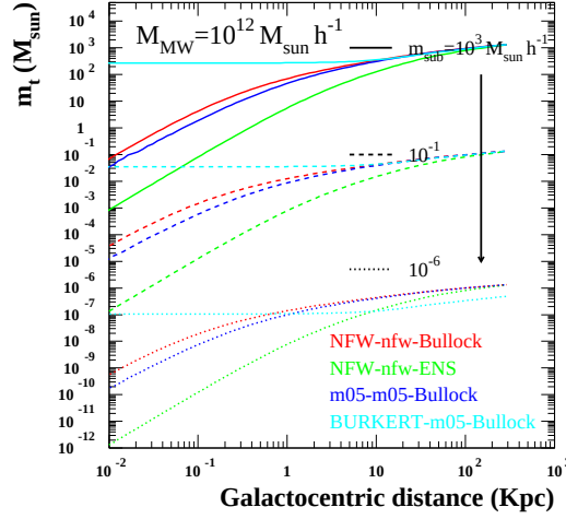
Figure 2.5: Masses within the tidal radius against the distance from the center of the Milky Way, for the same models of Fig. 2.4. Figure by Bisesi & Ullio, 2006 [42].
